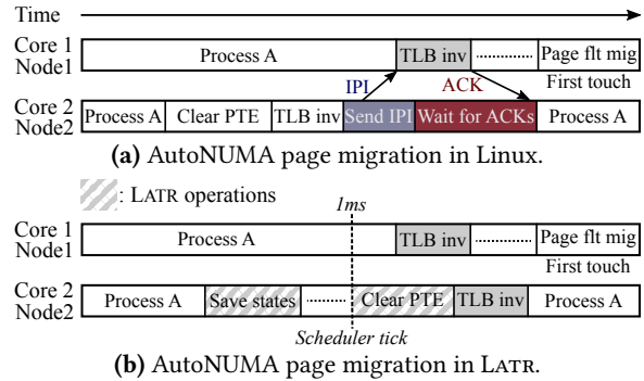
Figure 3. AutoNUMA page migration in both Linux and LATR. LATR removes the need for an immediate TLB shutdown when sampling pages for NUMA migration.
